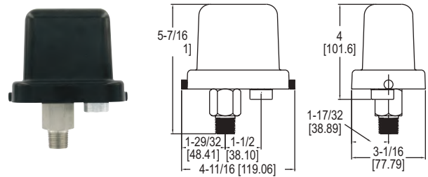
A1F with -PC weatherproof housing
