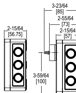
Duct mount
