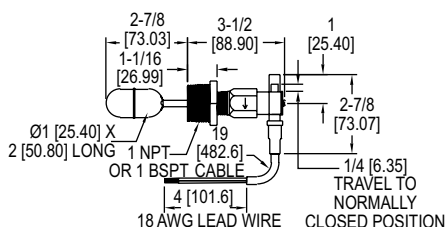
Cylindrical float
