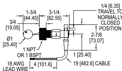
Spherical float
